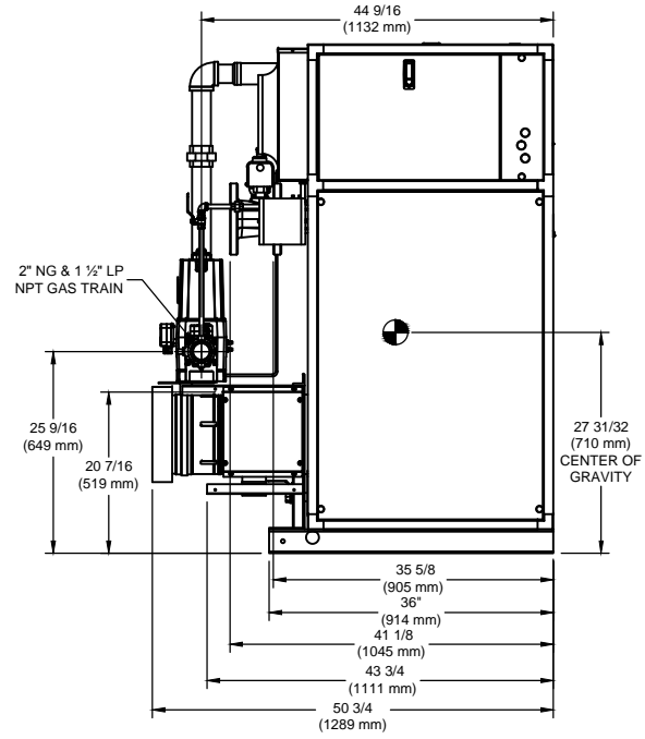
LEFT VIEW
